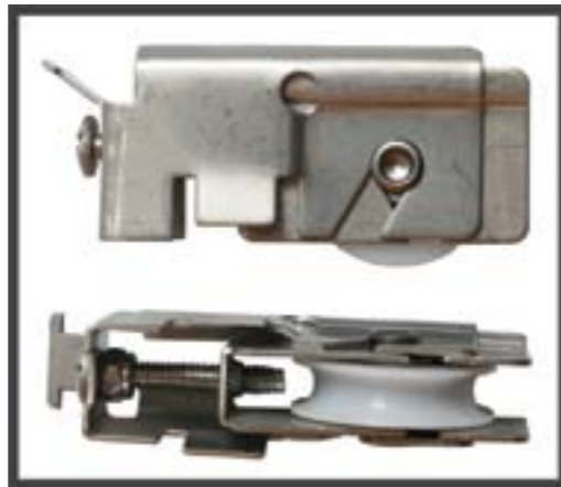
Roller 18mm PDR01SS
